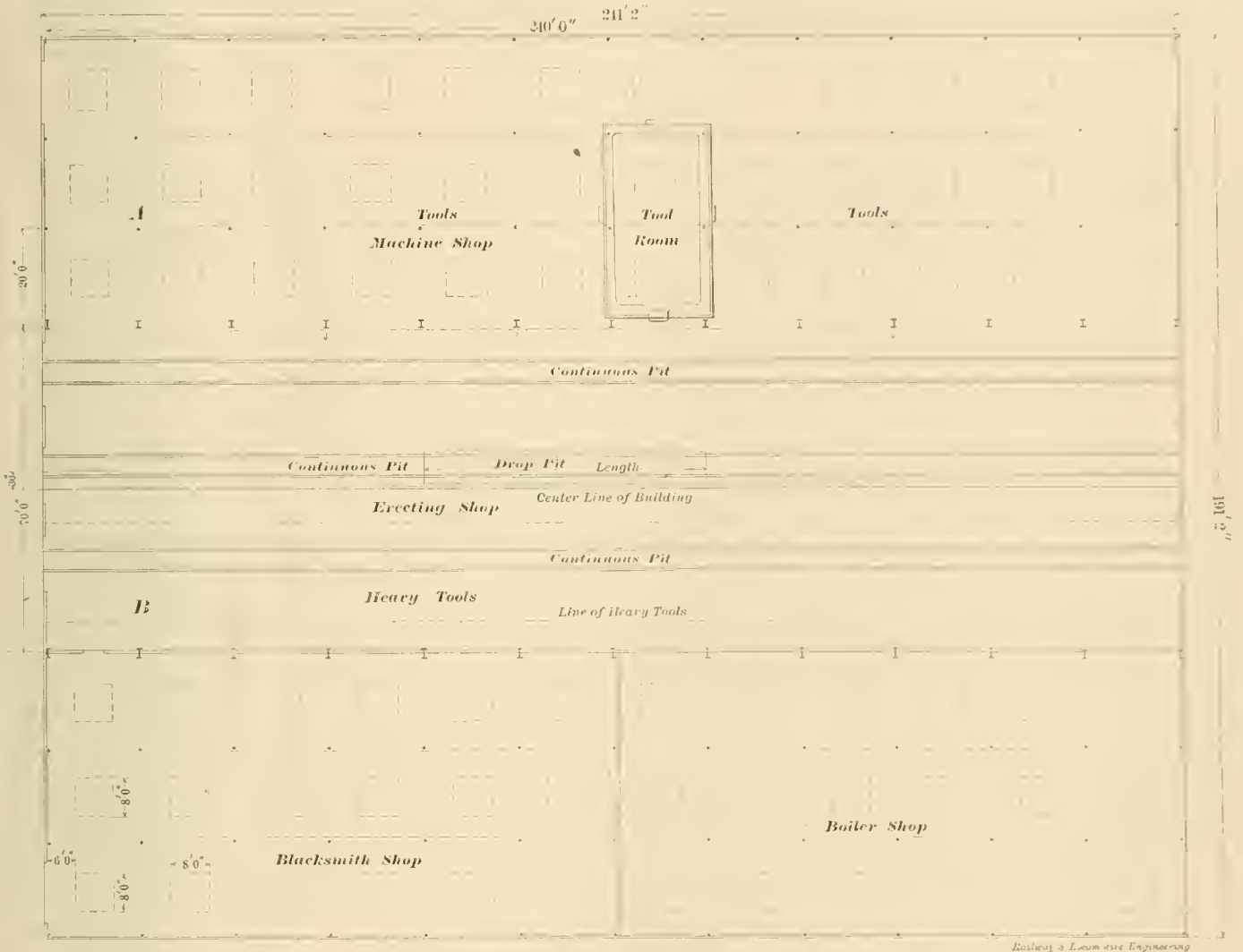
PLAN OF ERIE MACHINE, ERECTING, BOILER AND BLACKSMITH SHOPS.
